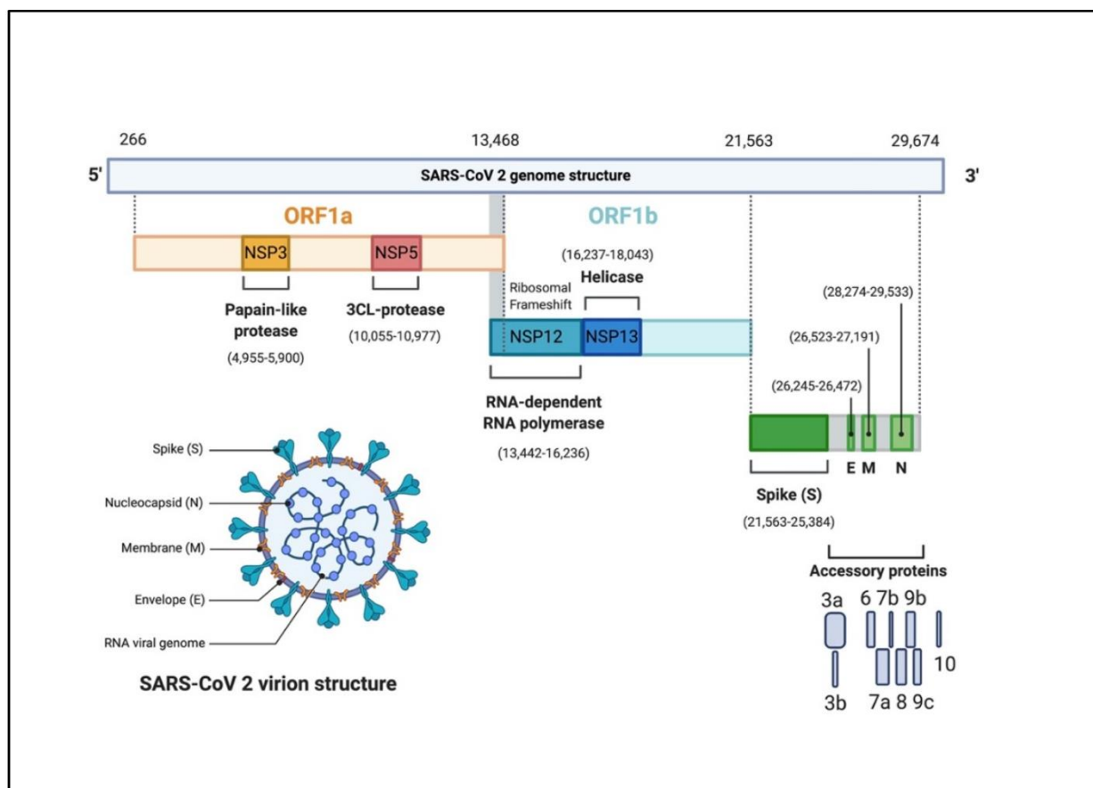
Рис.2 – генетическая структура SARS-CoV-2 (no: Alanagreh, Foad Alzoughool, Manar Atoum, 2020[3])
